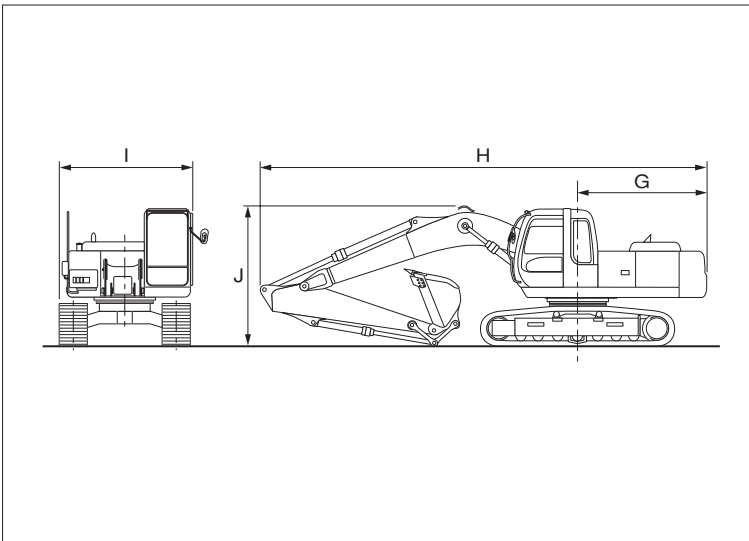
ZAXIS200
